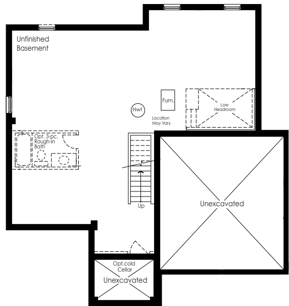
Basement Elev. A, B & C
